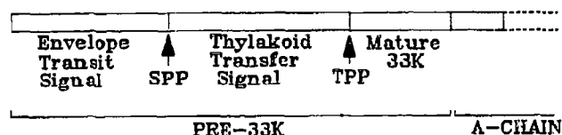
Fig. 1. Structure of the 33-RA fusion protein. 33-RA consists of the 33K pre-sequence (79 residues) together with 22 residues of mature 33K protein, followed by linker peptide (boxed) Glu-Asp-Asn-Asn and mature A chain (open dashed line). The 33K pre-sequence contains 2 targeting signals in tandem: an envelope transit signal, which is removed by a stromal processing peptidase (SPP), followed by a thylakoid transfer signal which is removed by a thylakoidal processing peptidase (TPP).
